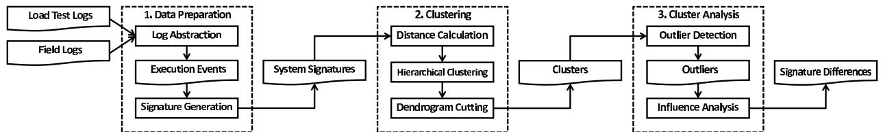
Figure 1: An Overview of Our Approach.
