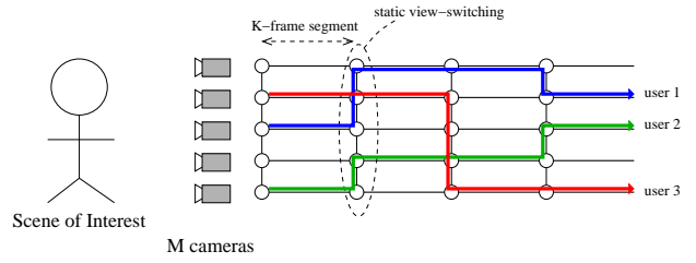
Fig. 1. In an IMVS scenario with static view-switching, different users select different view trajectories in the high-dimensional media space.
