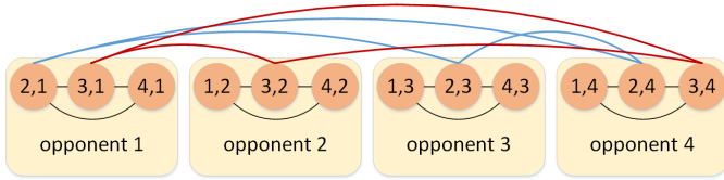
Fig. 1. Example of four subgraphs connected to a large graph for four teams. Intra-subgraph edges are black, and inter-subgraph edges are blue or red for team 2 and 3 respectively.
