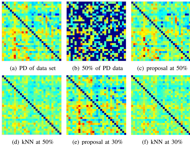
Fig. 2. Missing entries prediction on NBA data set. (a) shows the ground truth game differentials for pairs of teams. (b) shows game differentials with 50% of entries removed. (c) and (d) show the predicted game differentials for our proposal and kNN when 50% of data are missing. (e) and (f) show the predicted game differentials for our proposal and kNN when 30% of data are missing.
