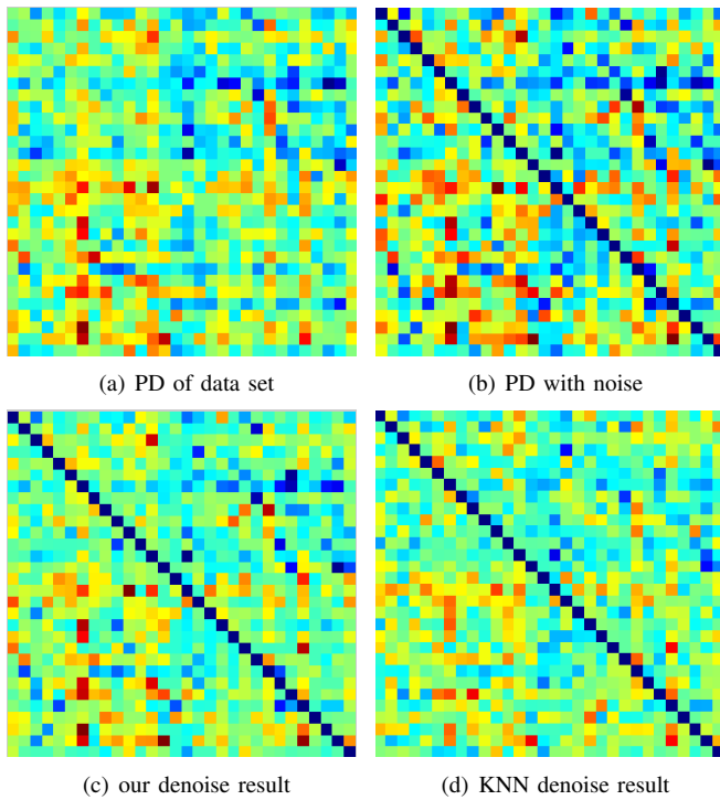
Fig. 3. Denoising on NBA data set. (a) shows the ground truth game differentials for pairs of teams. (b) shows the noise corrupted game differentials. (c) shows the denoised game differentials for our proposal. (d) shows the denoised game differentials predicted for kNN.
