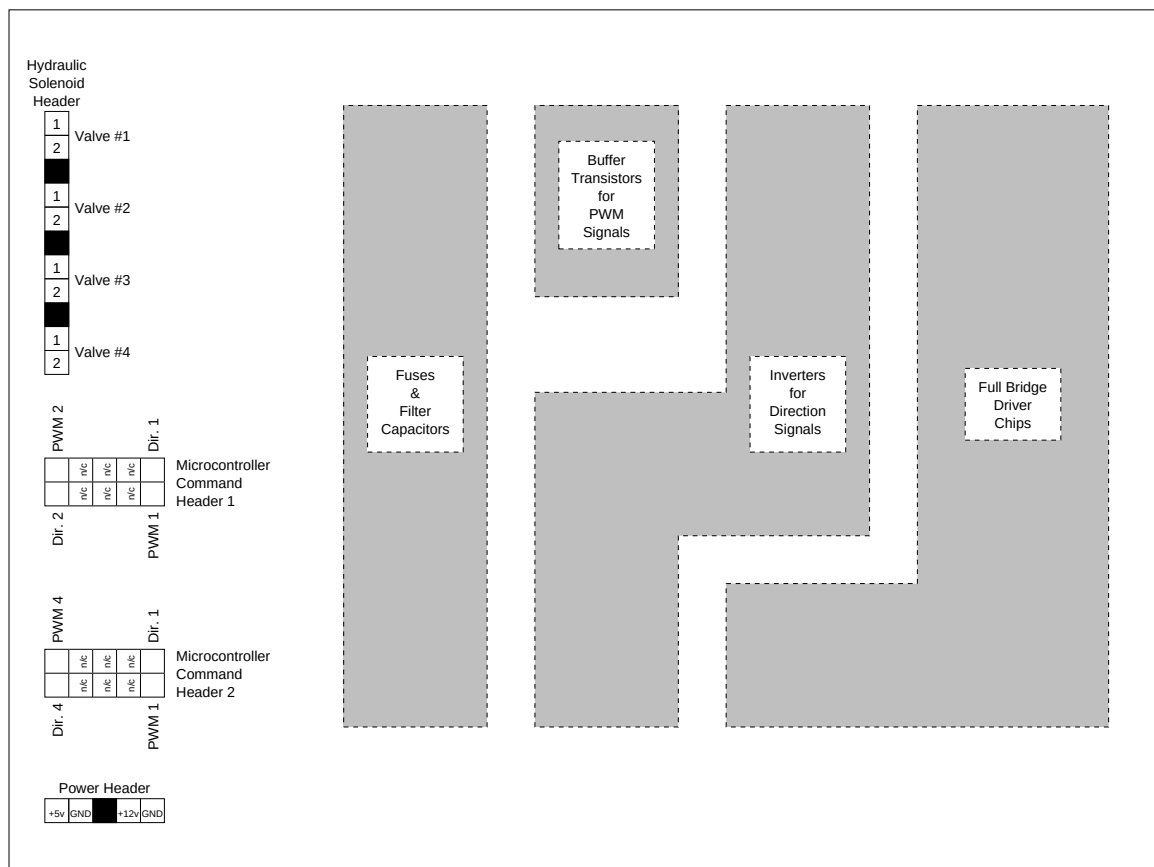
Figure 2.12: Low current driver board Layout.
