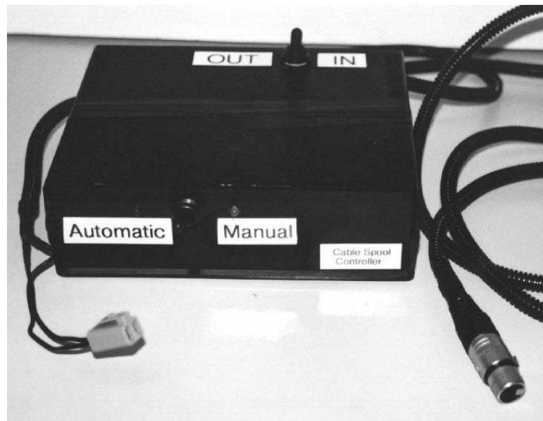
Figure 2.9: Outside Spool Control.
