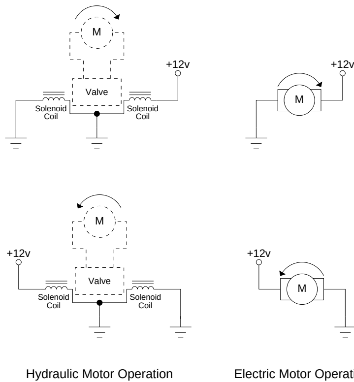
Figure 2.4: Electric operation of the hydraulic valve system versus a similar DC motor system.
