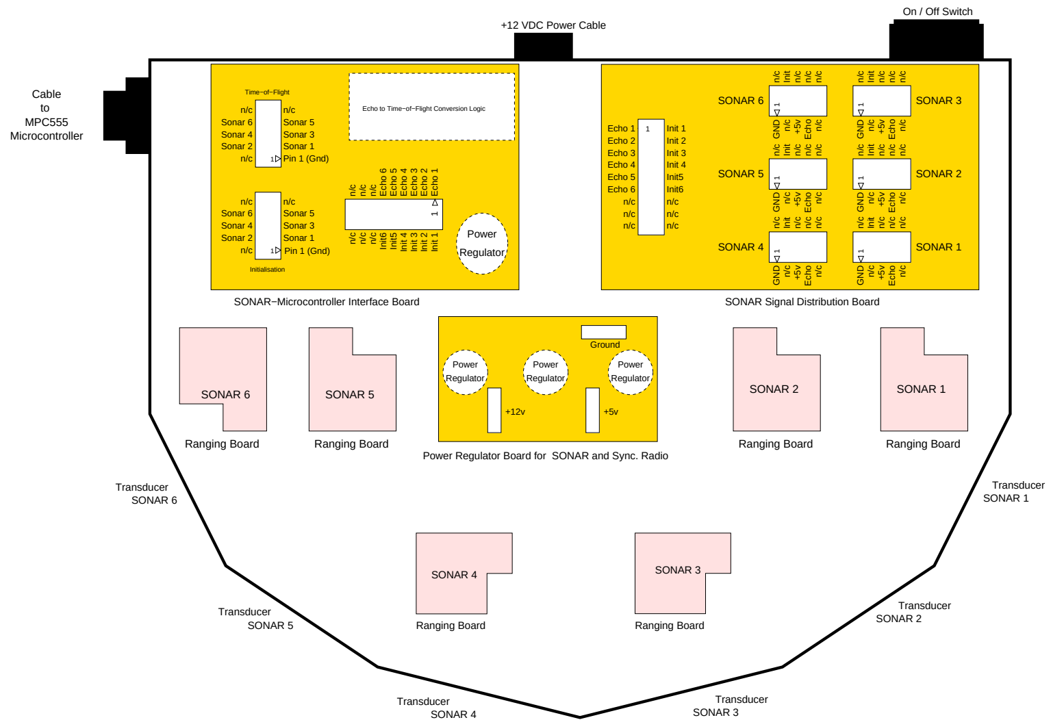
Figure 3.13: SONAR Array board layout
