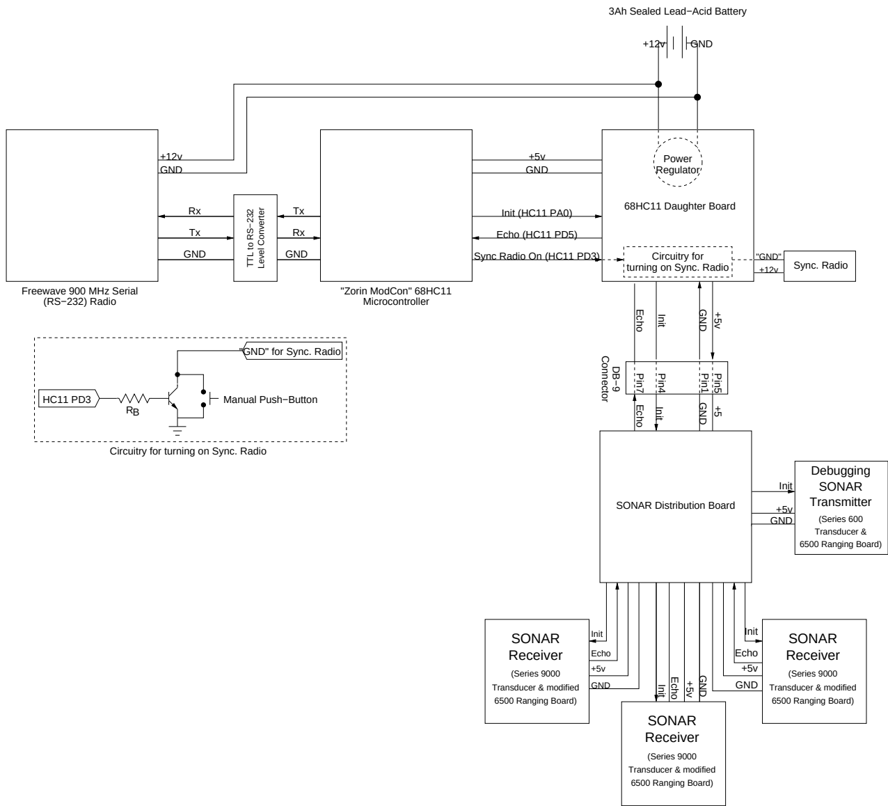
Figure 3.17: The Pursuit Pack Component Block Diagram.
