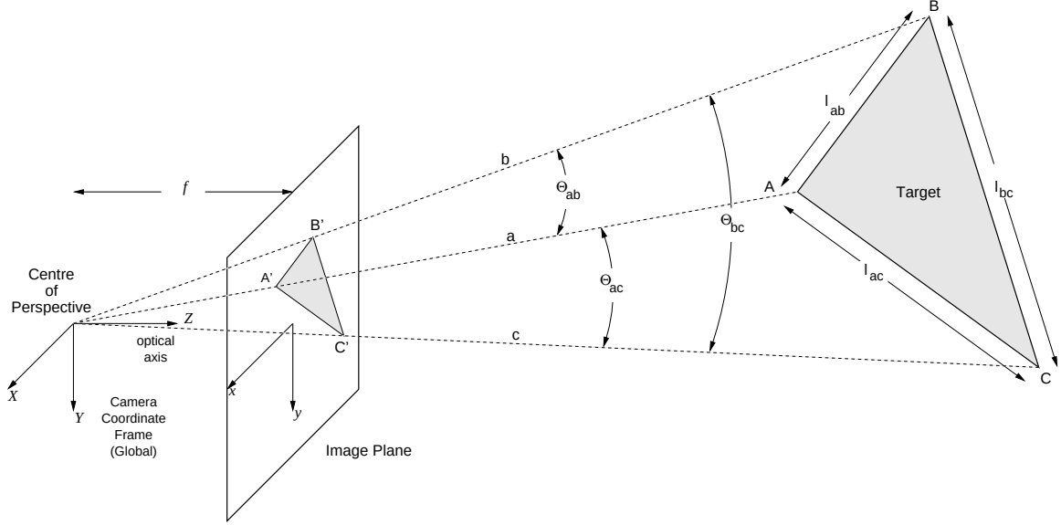
Figure 3.4: Variables used in Perspective-3-Point calculations.
