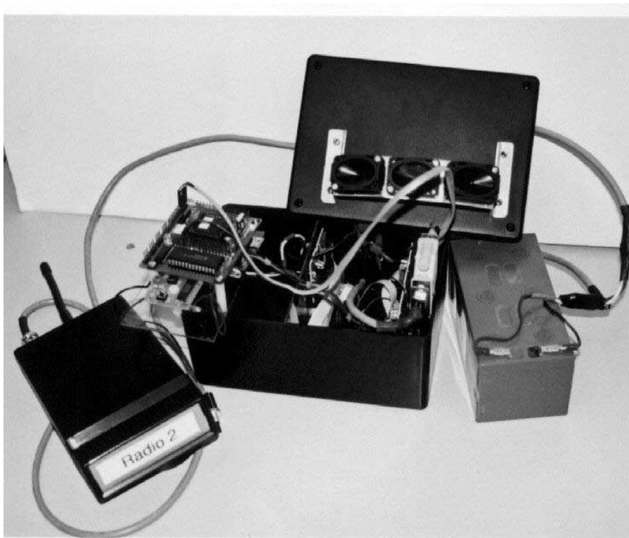
Figure D.5: The Pursuit Pack Components. Micro-controller removed from box.
