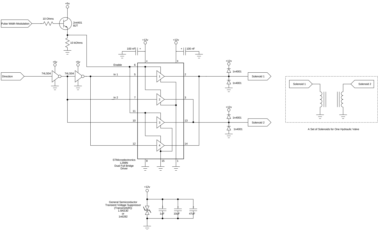
Figure 2.11: Schematic for one of four identical low current solenoid driver circuits.
