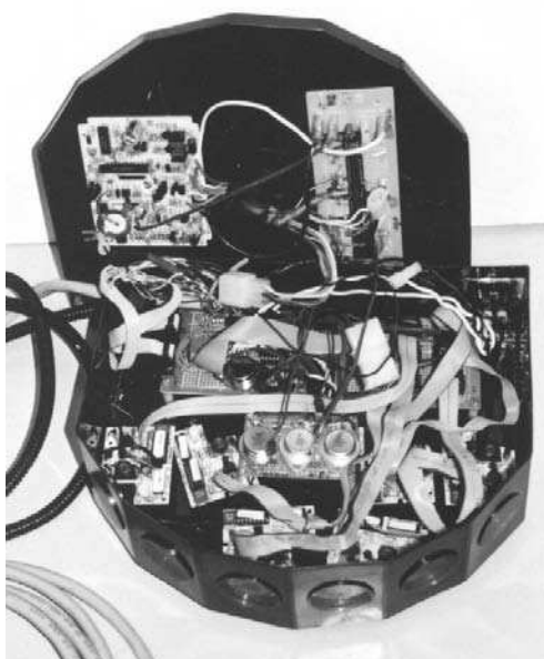
Figure 3.15: Inside SONAR Array. Note the radio synchronisation electronics attached to the Array's lid while the SONAR array electronics are at the bottom.
