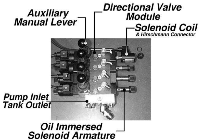
Figure 2.5: The Hydraulic Valve Deck.
