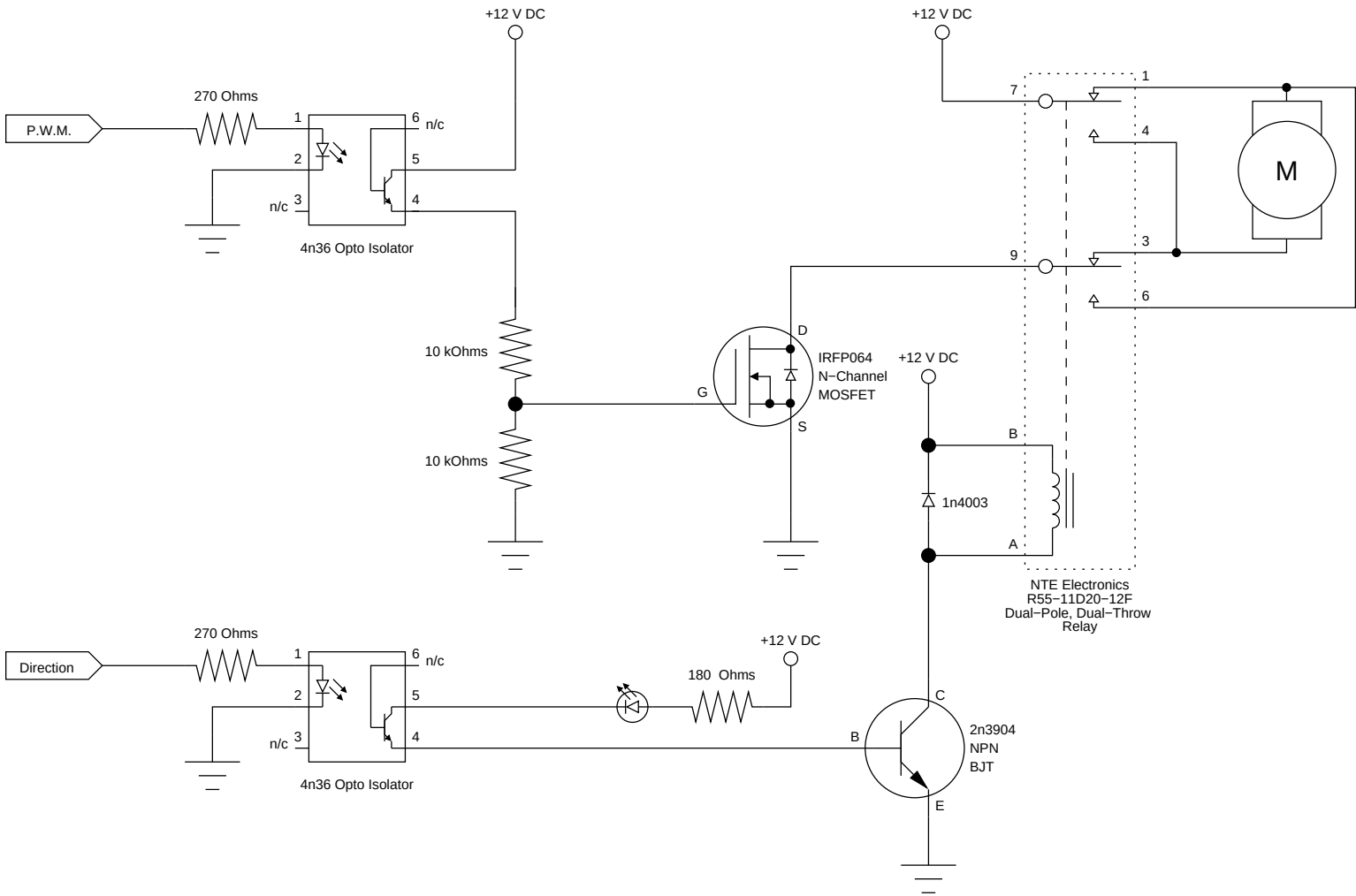
Figure 2.7: Mixed Transistor-Relay Motor Driver.
