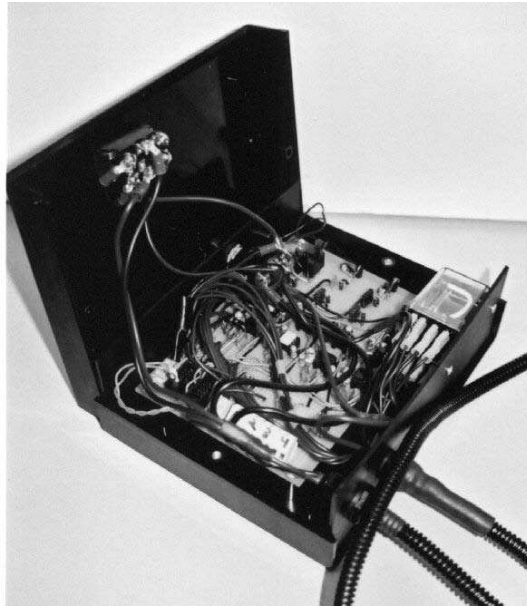
Figure 2.8: Inside Spool Control, featuring Mixed Transistor-Relay Driver.
