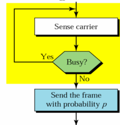
Persistent strategy
