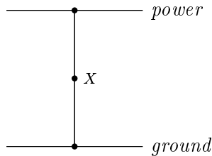
Figure 12.5: Short circuit
