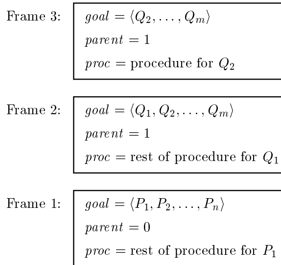
Figure 15.2: Stack layout
